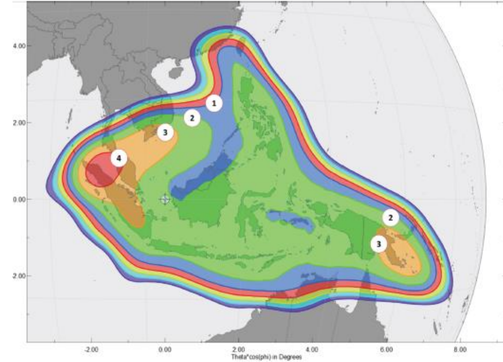
G/T C-Band South East Asia Beam
