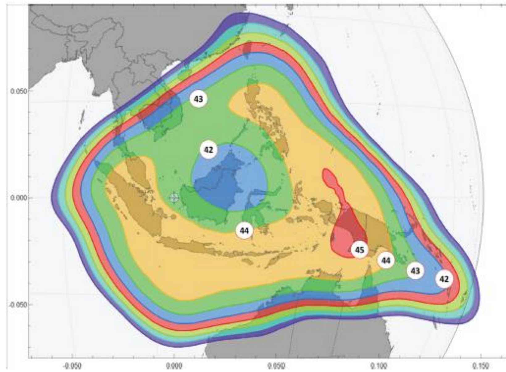
EIRP C-Band South East Asia Beam
